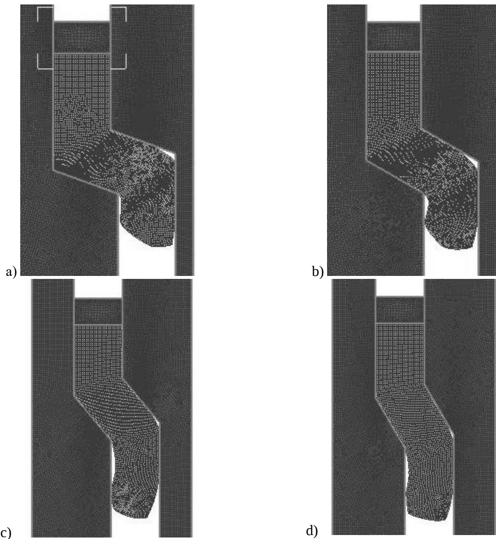
Figure 1– Equal-channel pressing in matrices of various designs: a – angular matrix with a channel junction angle 90^\circ ; b - angular matrix with a channel junction angle 130^\circ ; c - simple step matrix with a channel junction angle 130^\circ ; d - step matrix with rollers and a channel junction angle 130^\circ .
