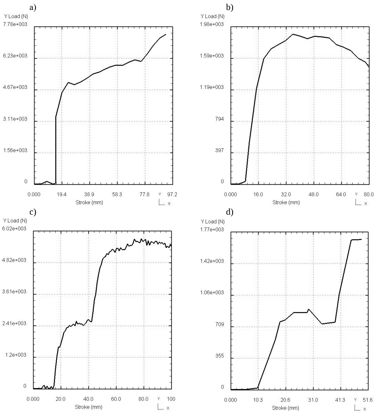
Figure 4 – Graphs of changes in deformation forces depending on the stroke of the punch in matrices of various designs: a – angular matrix with a channel junction angle 90°; b – angular matrix with a channel junction angle 130°; c - simple step matrix with a channel junction angle 130°; d - step matrix with rollers and a joint angle channels 130°.
