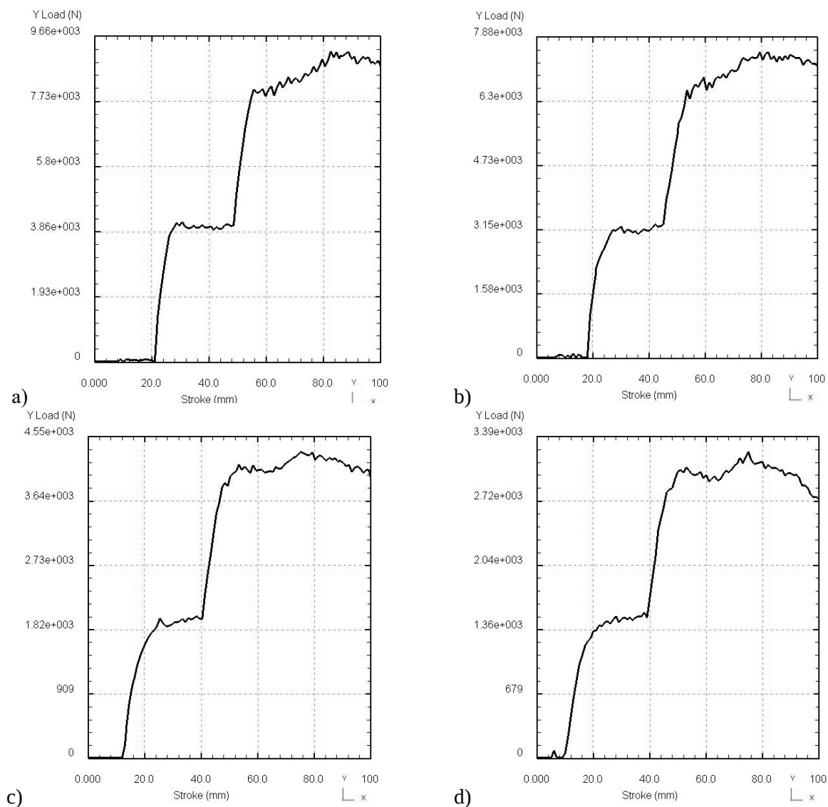
Figure 5 – Graphs of the change in deformation forces depending on the punch stroke at different angles of the channels junction of the step matrix: a – 110^\circ ; b – 120^\circ ; c – 140^\circ ; g – 150^\circ
