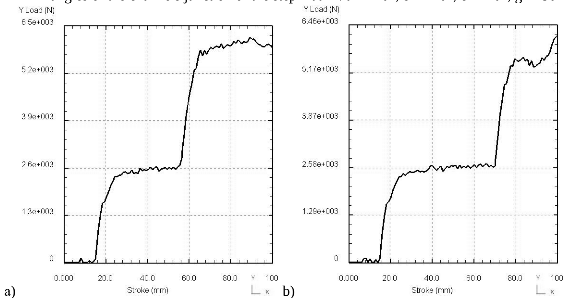
Figure 5 – Graphs of the change in deformation forces depending on the punch stroke at different angles of the channels junction of the step matrix: a – 110^\circ ; b – 120^\circ ; c – 140^\circ ; g – 150^\circ
